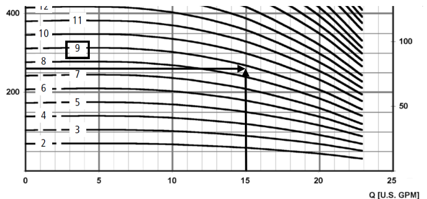
Pump performance curve
